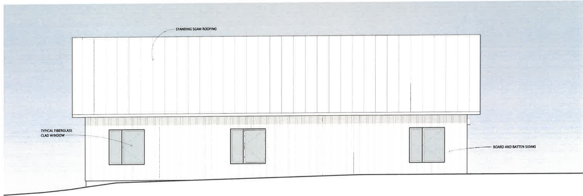
2 PROPOSED BUILDING ELEVATION - EAST SCALE: 1/4" = 1'-0"
